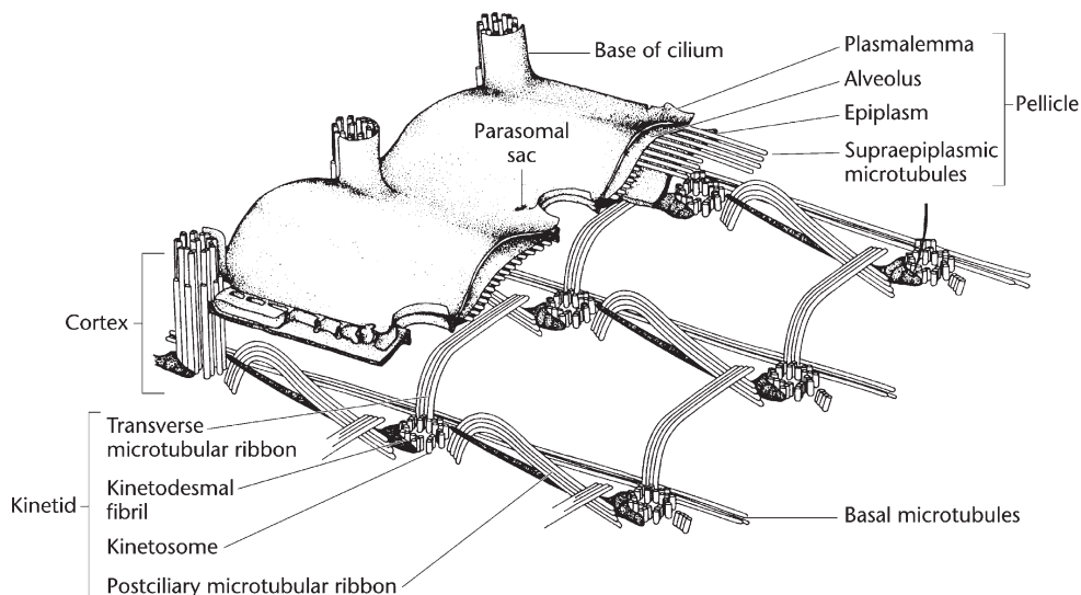
Figure 3 A patch of the cortex of a ciliate that shows the subcomponents of the pellicle and the kinetid. The microtubular and filamentous components of the cortex are elements of the cytoskeleton that provide support for the form of the ciliate. Based on Lynn and Small (1989).
