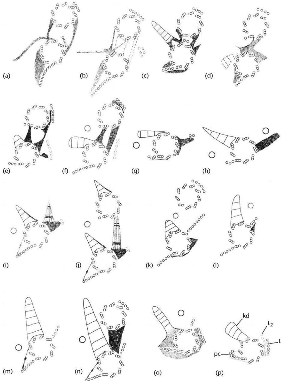
Figure 4 Transverse sections of the somatic kinetids of representative genera from the major classes of ciliates. (a, b) Subphylum Postciliodesmatophora. (a) Class Karyorelictea – Geleia . (b) Class Heterotrichea – Climacostomum . (c–p) Subphylum Intramacronucleata. (c, d) Class Spirotrichea – Protocruzia (c) and Stylonychia (d). (e, f) Class Colpodea – Sorogena (e) and Pseudoplathyphrya (f). (g, h) Class Phyllopharyngea – Hypocoma (g) and the suctionian Trichophrya (h). (i, j) Class Nassophorea – monokinetid (i) and dikinetid of Nassula (j). (k, l) Class Oligohymenophorea – dikinetid of Colpidium (k) and monokinetid of Ichthyophthirius (l). (m, n) Class Prostomatea – monokinetid (m) and dikinetid of Coleps (n). (o, p) Class Litostomatea – Lepidotrachelophyllum (o) and Isotricha (p). kd, kinetodesmal fibril; pc, postciliary microtubular ribbon; t1 and t2, transverse microtubular ribbons. Based on Lynn (1996a).
