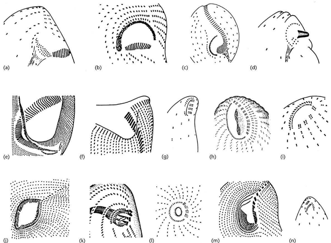
Figure 6 A demonstration of the diversity of oral structures of genera in the class Colpodea. Some of these ciliates represent oral features that are convergent on oral features of ciliates from other classes. (a) Colpoda with two oral polykinetids. (b) Hausmanniella also with two oral polykinetids. (c) Bardeliella with a left oral polykinetid that extends out over the anterior end as a series of rows of cilia. (d) Grossglockneria whose everted cytopharynx is used to pierce fungal cells and ingest their cytoplasm, like a suctorians' tentacle. (e, f) Bursaria (e) and Bursaridium (f) whose extensive series of left oral polykinetids placed them in the class Heterotrichea for many years. (g) Cyrtolophosis with its small number of oral polykinetids and small cell size was once considered a member of the class Oligohymenophorea. (h) Platyophrya with paroral and multiple left oral polykinetids. (i) Sagittaria similar to Platyophrya . (j) Rostrophrya with small polykinetids extending out on to the somatic surface was initially thought to be a member of the class Nassophorea. (k) Pseudochlamydonella whose ventral oral cavity and basket-like cytopharynx are similar to those structures in the class Phyllopharyngea. (l) Sorogena with its simple, ring-like anterior oral apparatus was initially classified as a member of the class Prostomatea. (m) Bryophrya shows some similarities to Rostrophrya and nassophoreans although it has a deep oral cavity. (n) Trihymena , a colpodean with a simple oligohymenophorean-like oral apparatus. Based on Lynn (1996a) and Foissner (1993).
