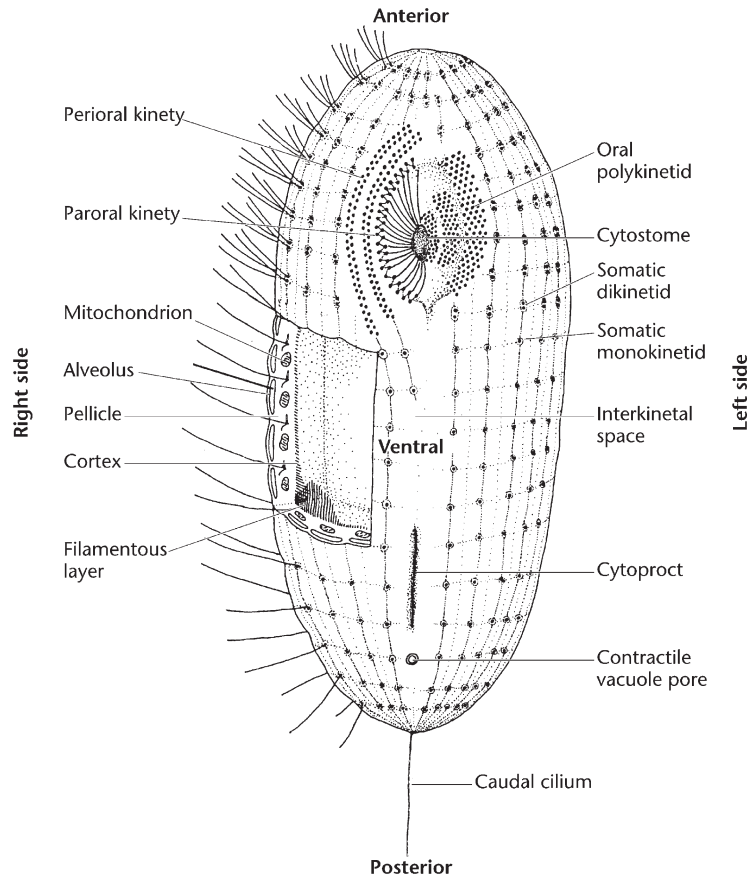
Figure 2 Generalized drawing of the ventral surface of a ciliated protozoan. The body can be divided into somatic and oral regions. The oral region illustrated here has two oral polykinetids and one paroral kinety, and adjacent to this are some specialized perioral kineties that aid in feeding. Refer to Figure 6 for some illustrations of more oral structures. The somatic cortex is covered by a pellicle that includes the alveoli (see Figure 3). The pellicle is part of the cortex, the outer portion of the cell in which are embedded the somatic mono- and dikinetids and the mitochondria. The cortex may be separated from the endoplasm by a filamentous layer. There are typically three openings to the outside: the cytostome or cell mouth through which food passes into the food vacuole; the cytoproct through which undigested food passes from the food vacuole and the contractile vacuole pore out of which excess water and some wastes are passed from the contractile vacuole. Based on Lynn and Small (1989).
