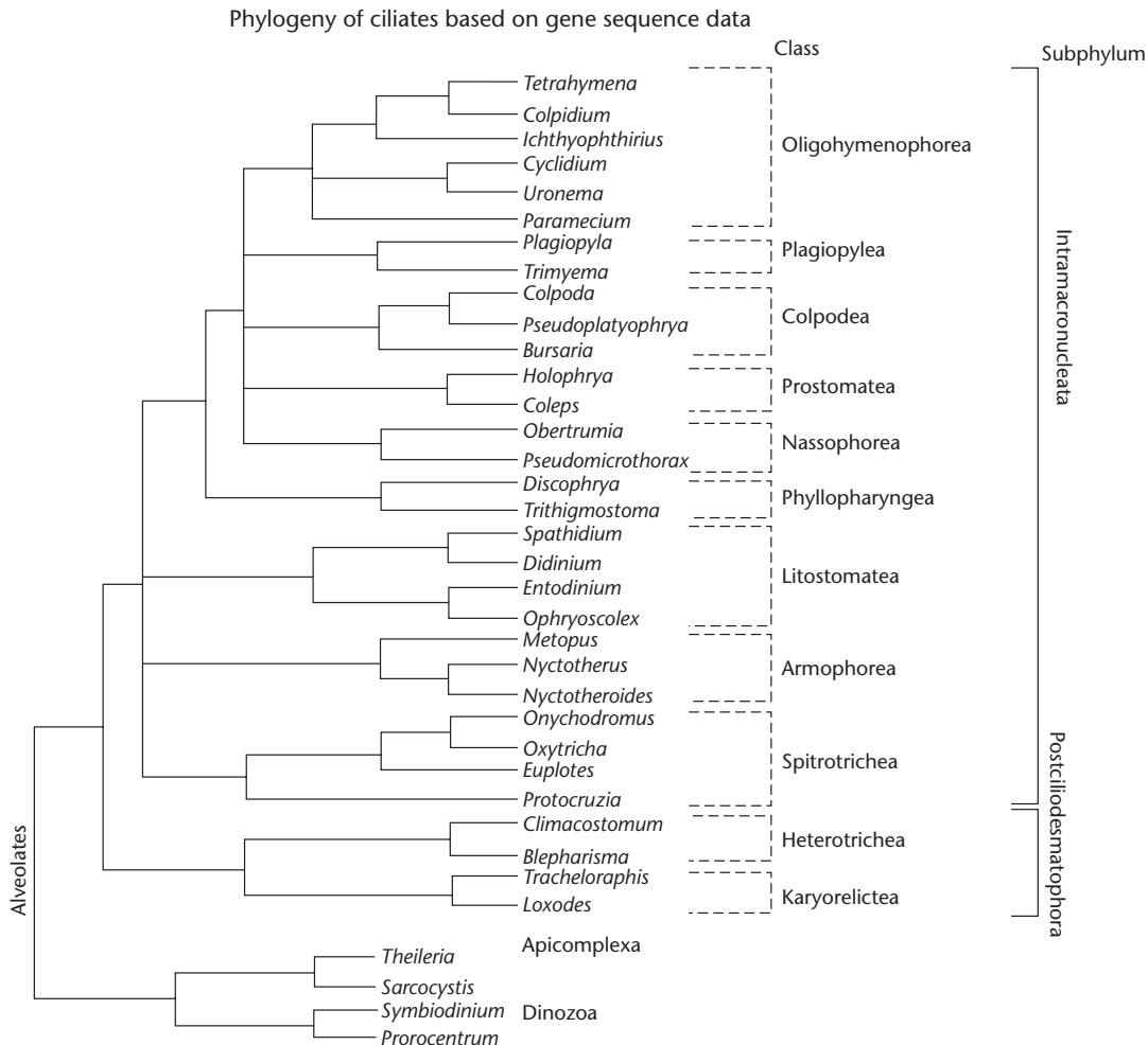
Figure 5 A phylogeny based on phylogenies derived from comparisons of the nucleotide sequences of ss-rRNA genes. The other two alveolate phyla Apicomplexa and Dinofzoa serve as outgroups to root the ciliate portion of the tree.
