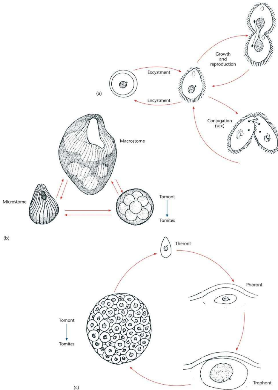
Figure 1 Life cycles of ciliated protozoa. (a) A generalized life cycle of a ciliate showing three major phases: (1) growth and reproduction during which the ciliate feeds and undergoes binary fission; (2) conjugation usually stimulated by starvation conditions, during which the ciliates undergo meiosis and exchange gametic nuclei before separating and (3) encystment and excystment during which the ciliate secretes a cyst wall about itself to survive harsh conditions, like desiccation or the absence of food. (b) The life cycle of the hymenostome Tetrahymena patula , which has a microstome phase that eats bacteria, a macrostome phase that eats microstomes and other smaller ciliates when the bacterial food supply is depleted and a tomont or dividing phase that undergoes sequential binary fissions in a cyst to produce tomites. The tomites escape the cyst when bacteria are again abundant. (c) The life cycle of the hymenostome Ichthyophthirius multifiliis , the parasite that causes white-spot disease of the skin of fishes. The theront, a small cell, burrows into the skin of a fish to become a phoront that begins feeding as a trophont stage. The trophont may reach over 1 mm in diameter at which time it falls off the fish on to the bottom to become a tomont. Here, the tomont divides sequentially by binary fission to produce sometimes 1000 tomites, which break out of the division cyst to become the next generation of theronts. Based on Lynn and Small (1989) and Lynn and Small (2002).
