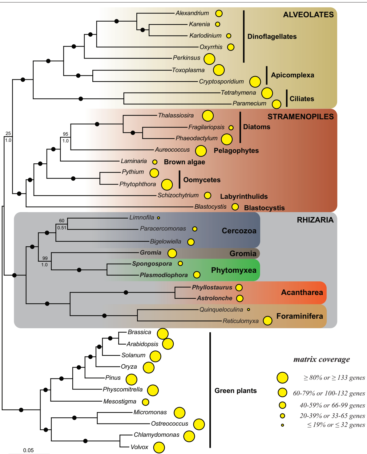
Figure 1 Phylogeny of SAR as inferred by RAXML and the LG model of evolution. The tree was rooted using the green plants. Species with new genomic data generated in this study are in bold. An identical topology was also recovered using MrBayes and the WAG model of evolution. Black dots correspond to 100% ML bootstrap support (BP) and 1.0 Bayesian posterior probabilities (PP). Numbers at nodes represent BP (above) and PP (below) when not maximal. The area of the yellow circles are proportional to the number of genes included in the supermatrix for each taxon. The scale bar represents the estimated number of amino acid substitutions per site.
