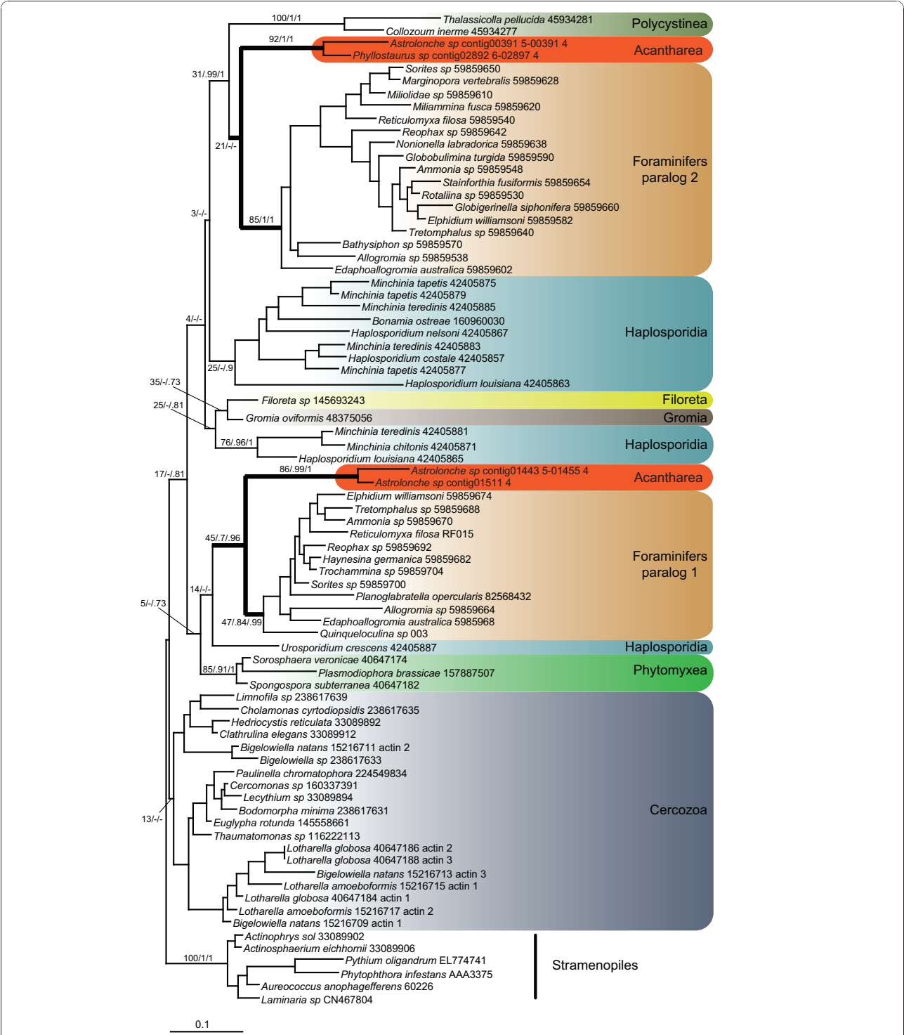
Figure 7 Actin phylogeny of Rhizaria. ML phylogeny of Rhizaria based on actin, rooted with stramenopiles as outgroup. Numbers at nodes represent the bootstrap values obtained with RAXML ("LG" model) and the posterior probabilities obtained with PhyloBayes ("LG" model) and MrBayes ("WAG" model). For clarity, only the values for the deep nodes and the nodes of interest for this study are shown. The scale bar represents the estimated number of amino acid substitutions per site. The branches leading to Acantharea and Foraminifera in actin paralogs 1 and 2 are in bold.
